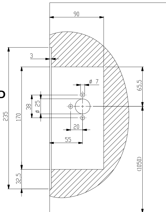
S9 MS LED
